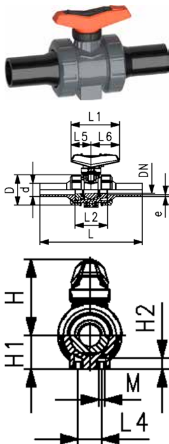
Ball valve type 546 pro With butt fusion spigots long PE100 SDR11 metric
