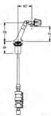
Short deck mount with loose hose barb
