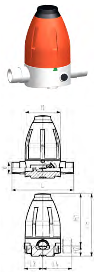
SYGEF Standard Pressure reducing valve type 582 With butt fusion spigots metric Without manometer
