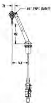
Deck mount dual head
