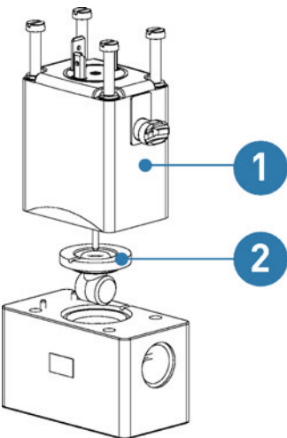
Wear part set (2) For solenoid valve type 157
